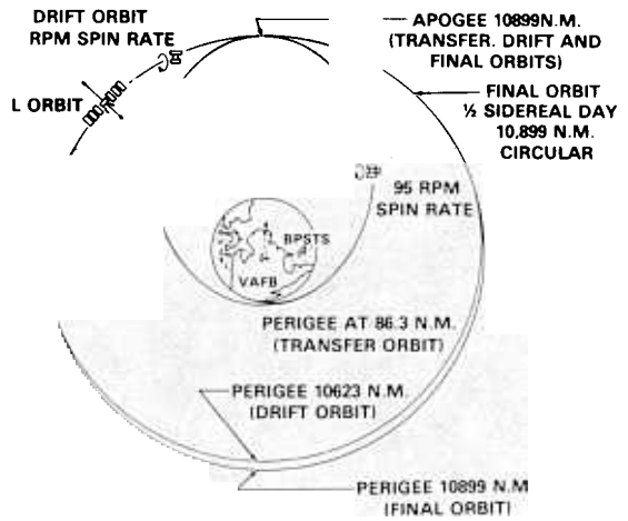
Fig. 3 - Mission sequence of NTS-2 events
