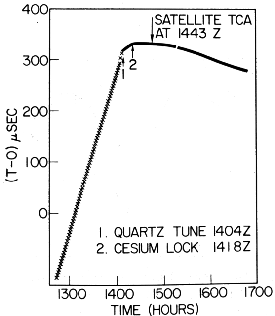
Fig. 19 - Cesium frequency standard lock up, 1977 day 190, 1418 UTC
