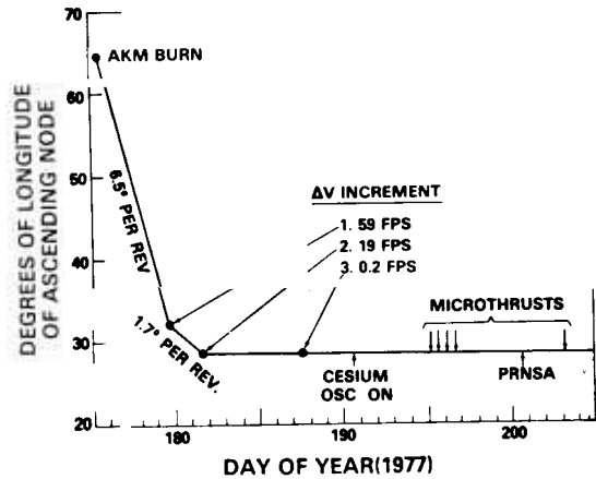
Fig. 9 - NTS-2 drift orbit adjustments
