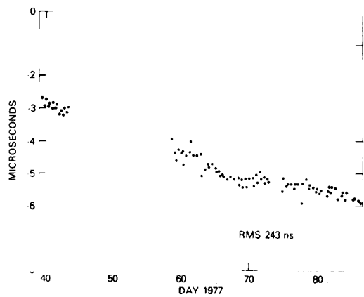
Fig. 29 - NTS-1 time transfer NASA Cape Kennedy Station
