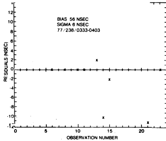
Fig. 39 - Laser residuals, Mt. Hopkins, 1977 day 238
