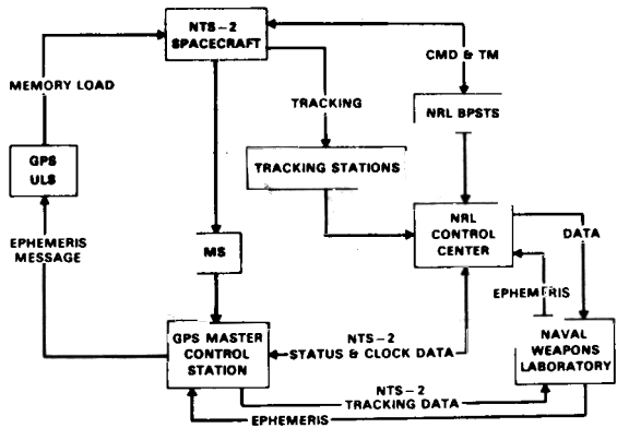
Fig. 7 - NTS-2 command and telemetry links
