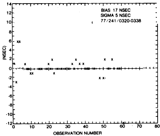
Fig. 40 - Laser returns, Mt. Hopkins, 1977 day 241
