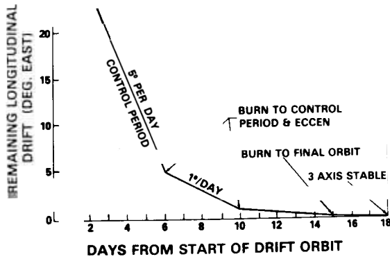
8 - Pre-launch NTS-2 drift orbit profile
