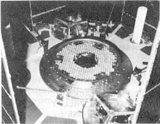
34 - NTS-1 laser retroreflector
