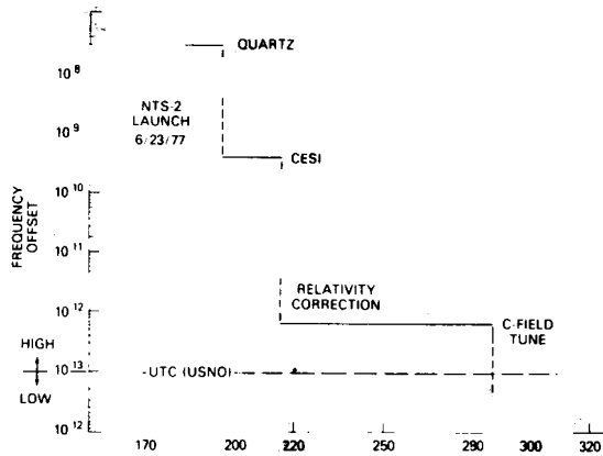
Fig. 27 - Frequency offset summary
