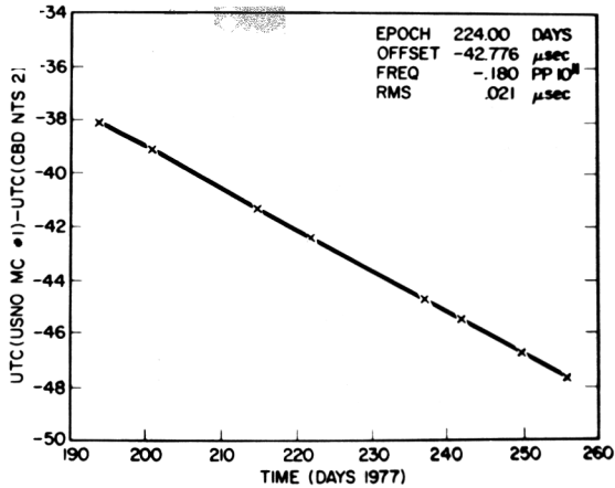
Fig. 22 - Frequency, USNO-CBD
