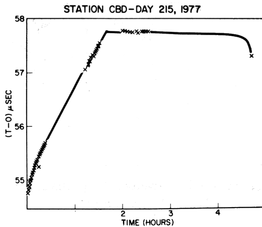
Fig. 21 - Effect of relativity correction
