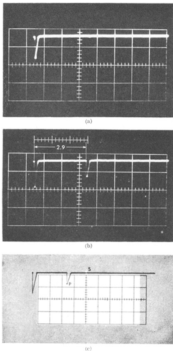
FIG. 4. (a) This photograph shows a single trace caused by a \mu -meson traversing the scintillator. Each major division of the time scale is one \mu sec. (b) This photograph shows a single trace caused by a \mu -meson stopping in the scintillator and decaying after 2.9 \mu sec. The ionization caused by the resultant electron produces the second pulse. (c) The drawing shows the position which the events recorded in 4(b) would have had during the experiment. The undeflected oscilloscope traces were behind the mask (shaded area) during the experiment. Only pulses (like P) from the decay electrons were visible. The small slit (S) in the mask was used to position the oscilloscope trace. A total sweep length of 8.5 \mu sec was used to detect the decay pulses.
